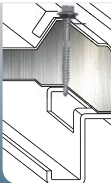
Crest Fixing
