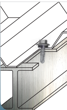
Valley Fixing
