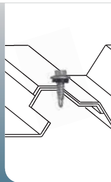
Stitching
